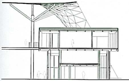
Type B Section B-B
