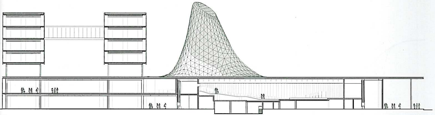
Services Center Section B-B'
