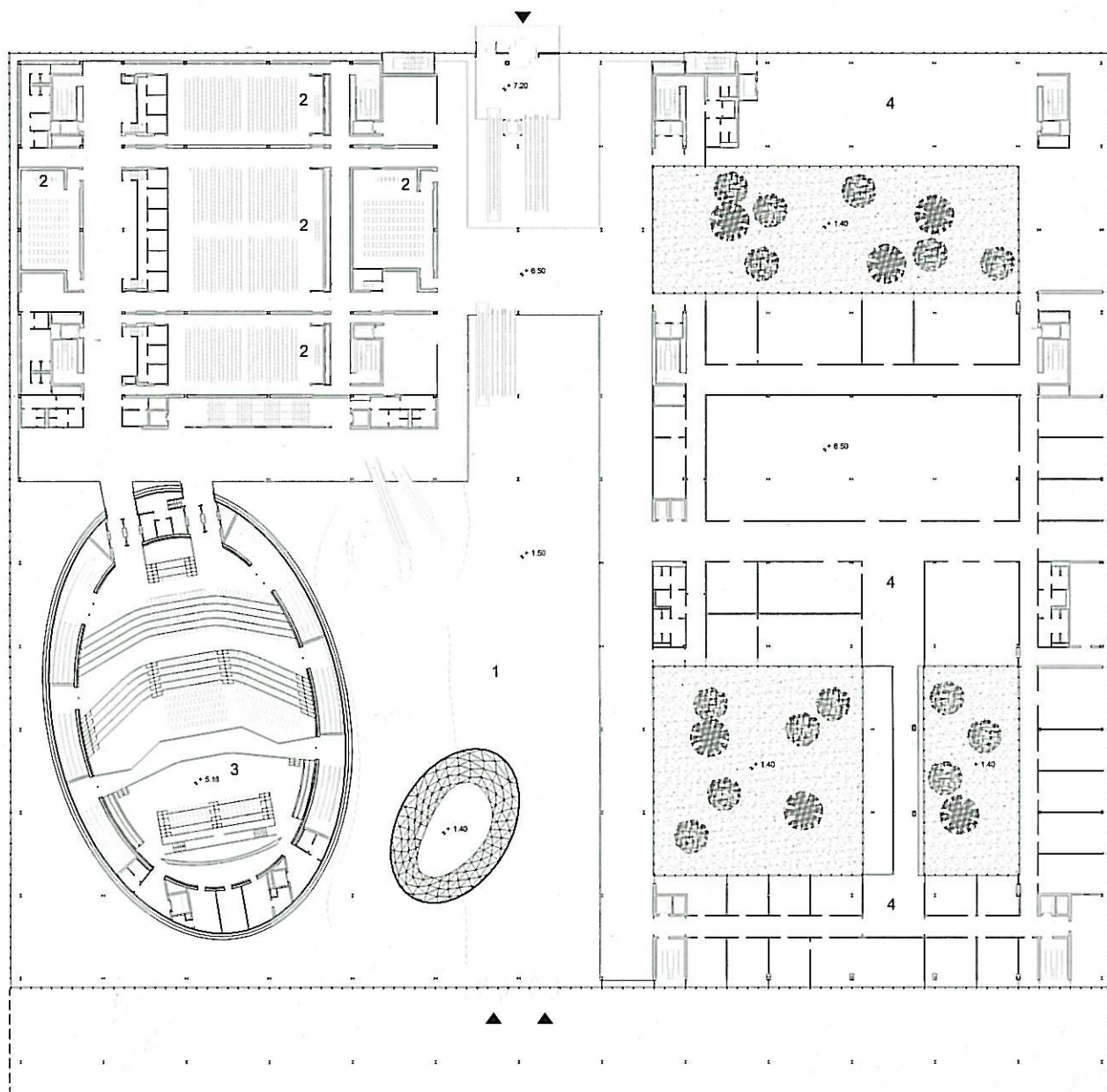
Services Center Plan +6.50
